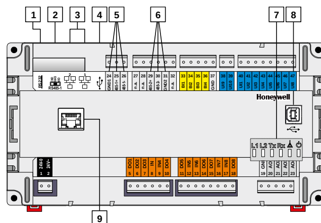
Figure 4: Top view (with HMI and a full complement of onboard I/Os)
