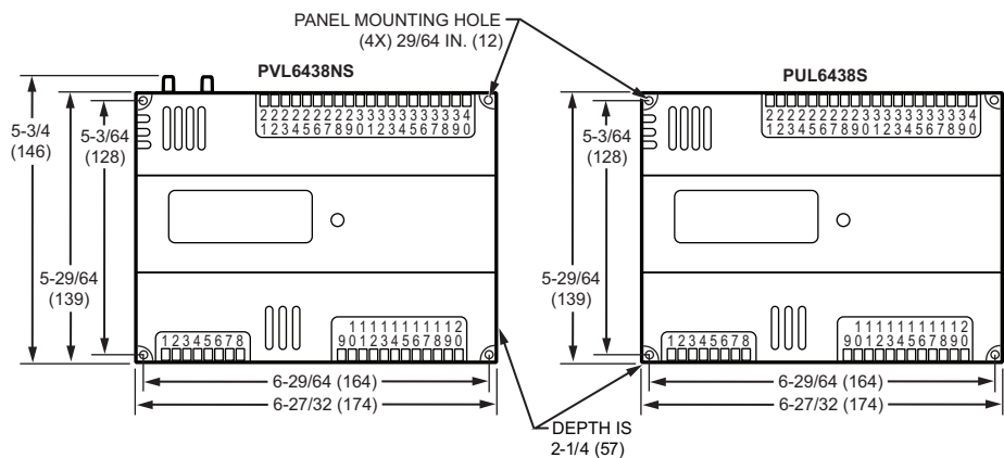
Fig. 7. Panel mounting - controller dimensions in inches (mm) for models PUL6438S and PVL6438NS only.
