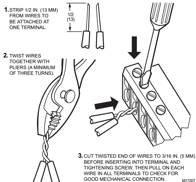
Fig. 15. Attaching two or more wires at terminal blocks.
