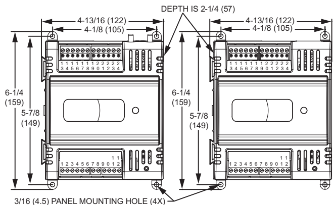
Fig. 6. Panel mounting - controller dimensions in inches (mm) for PUL1012S, PUL4024S, and PVL4024NS only (PUL4024S and PVL4024NS shown).
